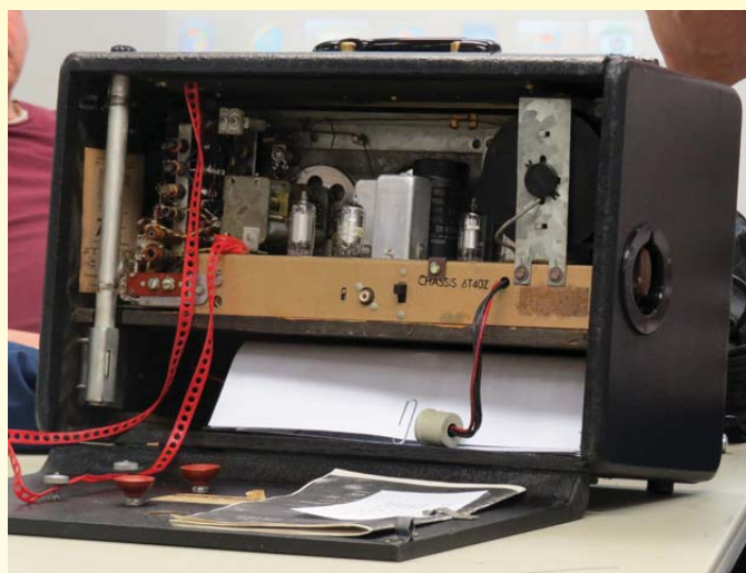
Above: rear view of the restored, early 1950's Zenith Transoceanic Radio. To the left: front view of the restored radio.
